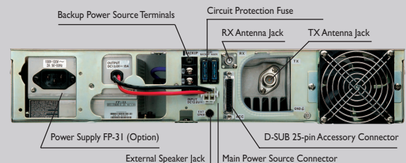
REAR PANEL
